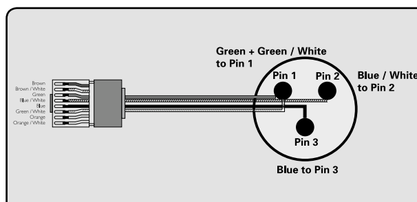
Figure 6.7.2b: XLR to RJ45 connections
