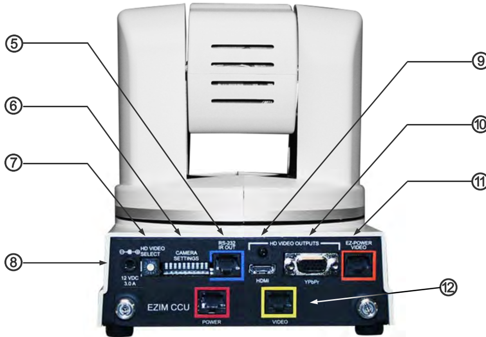
Image: PowerVIEW HD-20 or HD-30 HD PTZ Camera (Rear Panel) Rear Panel Connections with Feature Call-outs
