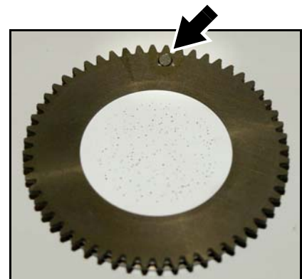
Figure 20: Goboholder magnet
