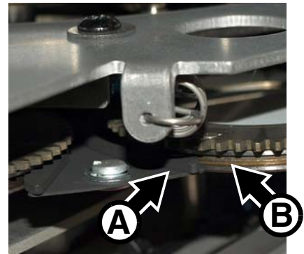
Figure 24: Gobo clip
