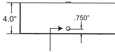
Single planished (.875" Dia) knockout for 1/2" conduit.
