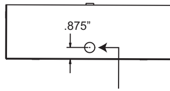
Single planished (1.11" Dia) knockout for 3/4" conduit.
