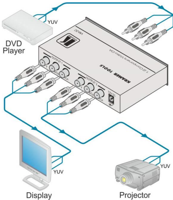
Figure 2: Connecting the VM-2C 1:2 Component Video DA
