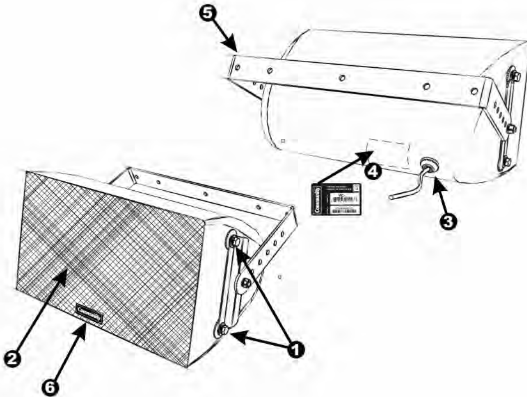
Figure 1 - Physical Features of a Typical Large WET II Enclosure
