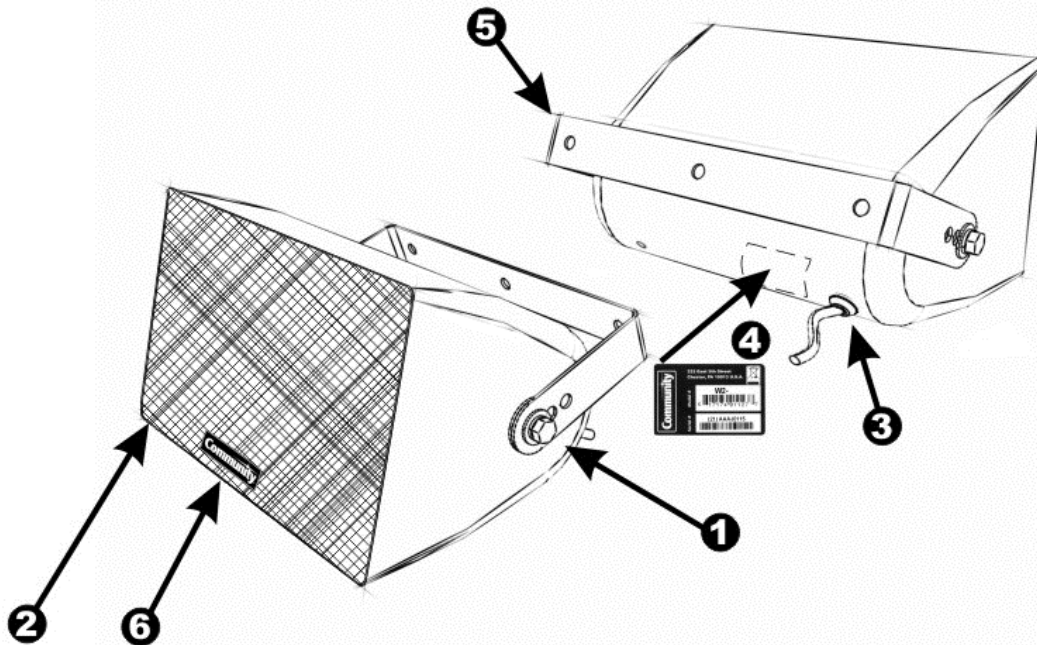
Figure 1 – Physical Features of a Typical Compact WET II Enclosure
