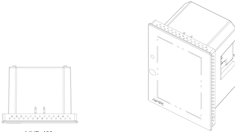
MXD-430 (Top View)
