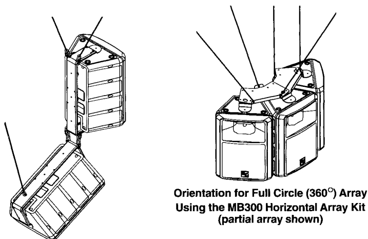
Vertical Array Using the Mb200 Installation Kit
