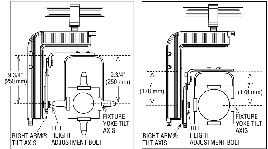
ETC Source Four Ellipsoidal ETC Yoke Measures 9 3/4" Adjust Tilt Arm To 9 3/4"
