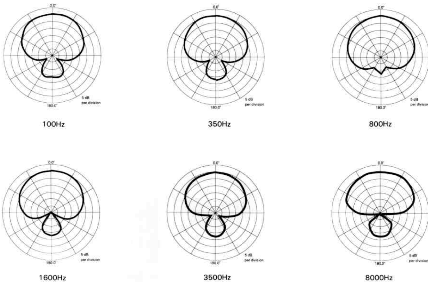
Polar Patterns Figure 1
