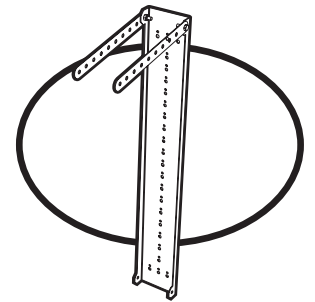
NXF35W with Angle Stand-Offs Attached (FIGURE 1)
