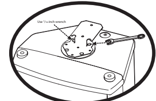
Bottom Plate Placement (FIGURE 2)
