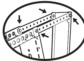
Using the Stand-Off Rails helps position the NX Enclosure at the perfect angle (FIGURE 4)
