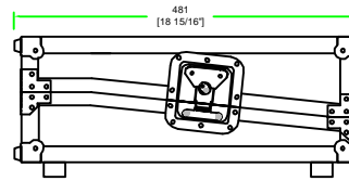
LEFT VIEW
