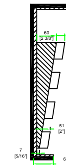
D-D VIEW
